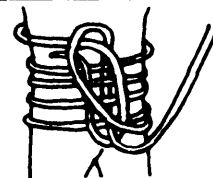
Bowline on a coil can be used by the first and last man on a climbing rope to take up unnecessary slack. A half-hitch must be employed behind the knot.
